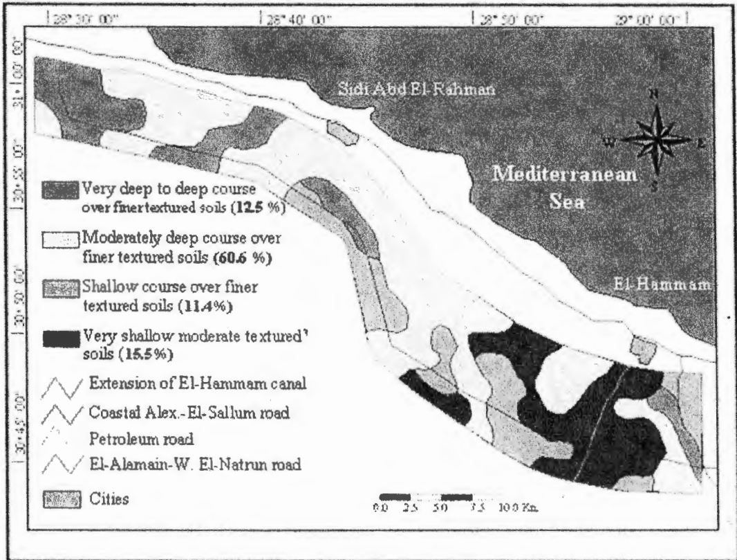
Map 3: Soil mapping units of the studied area
