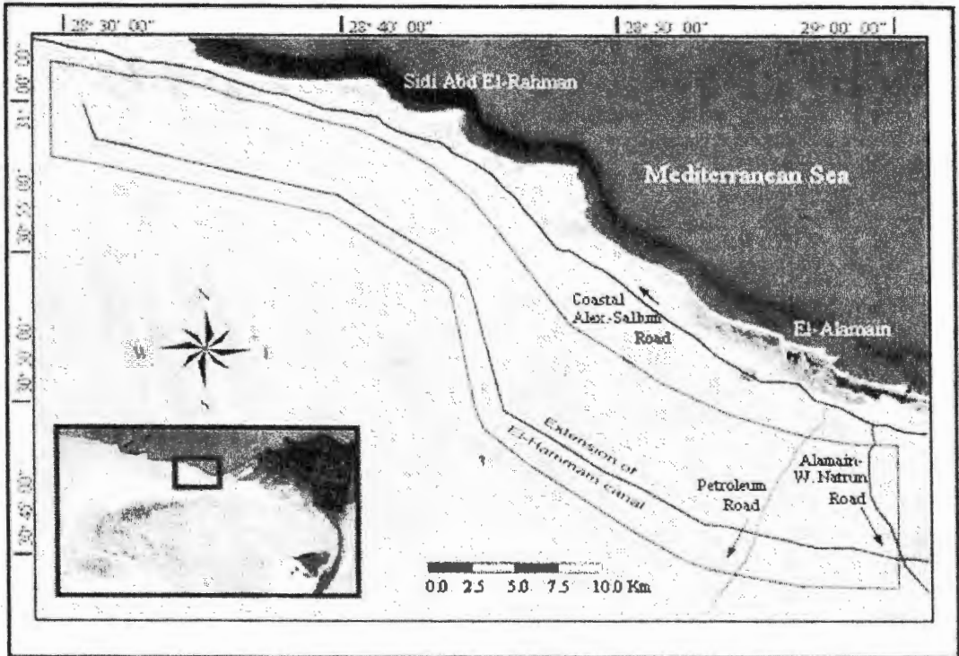
Map 1: Location of the studied area, North Western Coast of Egypt
