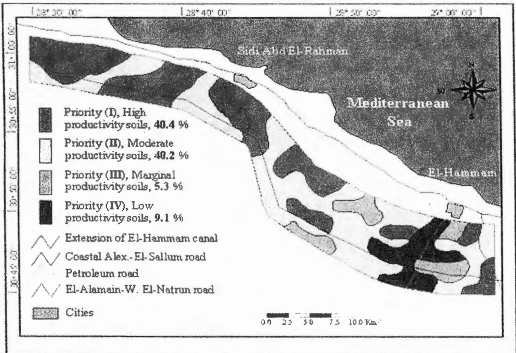
Map 4: Utilization priority based on land potentiality of the studied area
