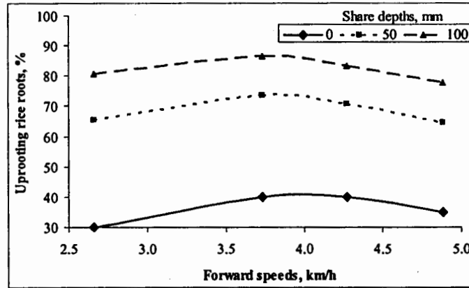
Fig. (14) Effect of forward speeds on uprooting rice roots at different share depths.
