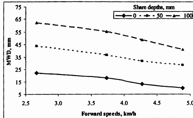
Fig. (4): Effect of forward speeds on MWD at different share depths
