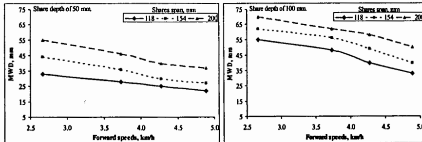
Fig. (3): Effect of forward speeds on MWD at different shares span and share depths
