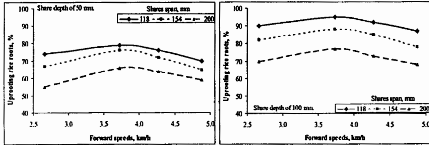
Fig. (13) Effect of forward speeds on uprooting rice roots at different shares span and share depths.
