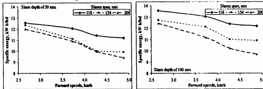
Fig. (9) Effect of forward speeds on specific energy at different shares span and share depths.
