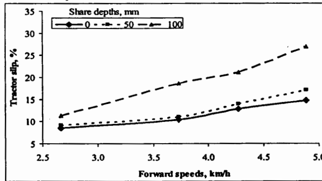
Fig. (8) Effect of forward speeds on tractor slip at different share depths.
