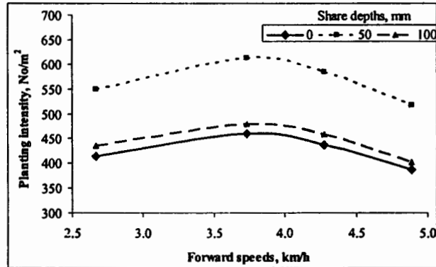
Fig. (12) Effect forward speeds on planting intensity at different share depths.
