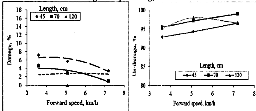
Link length reciprocating, C = 240mm
