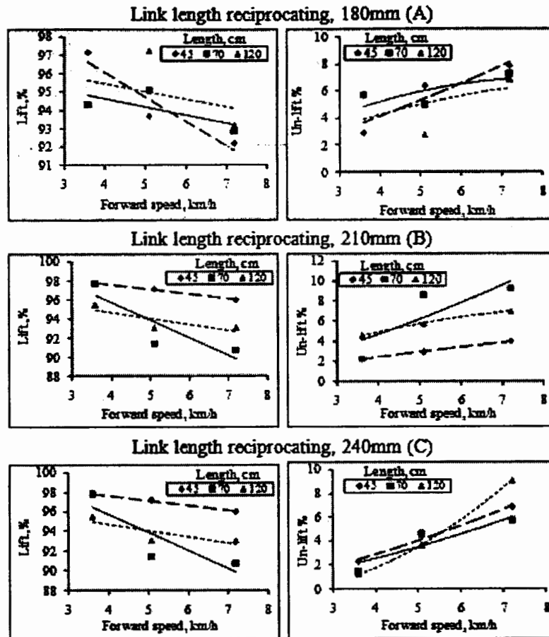
Figure (4): Effect of harvesting forward speed on lifted and un-lifted tuber
