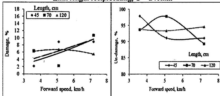
Figure (5): Effect of the harvesting forward speed on sweet potato
