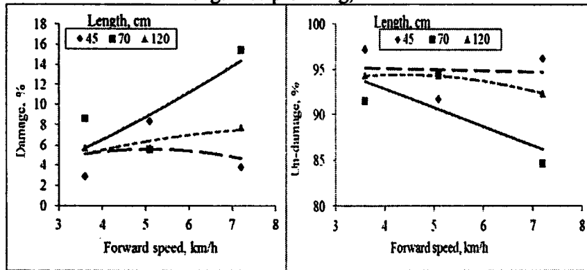
Link length reciprocating, A = 210mm
