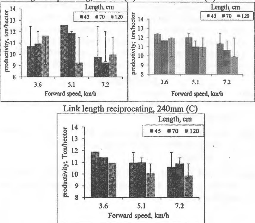
Figure (7): Harvesting forward speed via machine productivity
