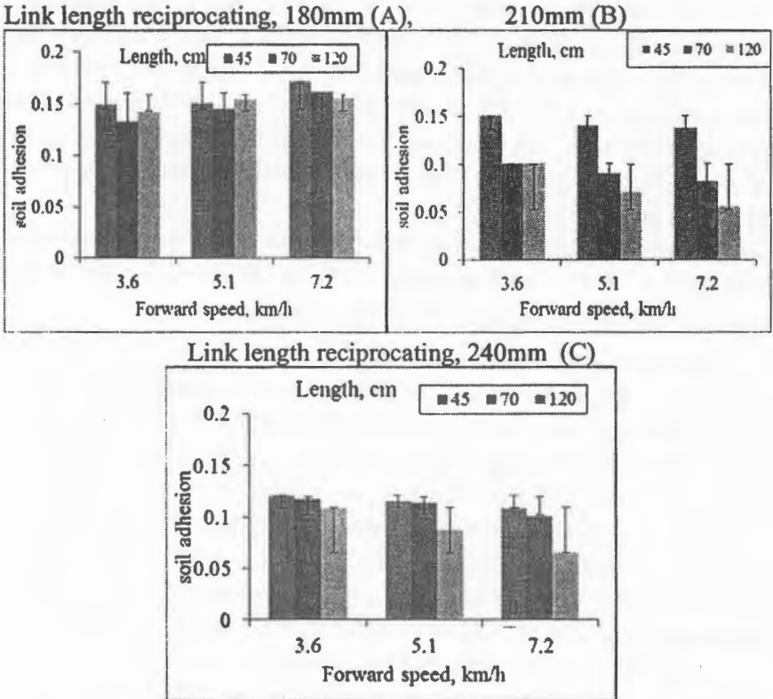
Figure (4-6): Harvesting forward speed via soil adhesion on sweet potato
