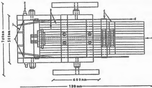
1- Share 2- Hatching points 3- Strips 4- Two longitudinal frames 5- Share frame 6- Separating unit
