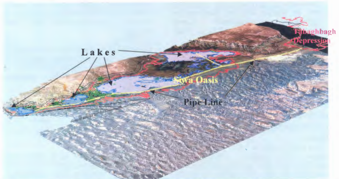
Fig 2: Proposed line to transfer disposing water from Siwa lakes to Tabaghbagh Depression over 3D Image, Siwa Oasis, Tabaghbagh, 2010.
