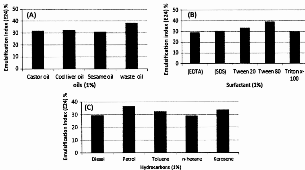
Fig. 4 Effect of different oils (A), surfactants (B) and hydrocarbons (C) on biosurfactant production by Streptomyces isolates 5S.
