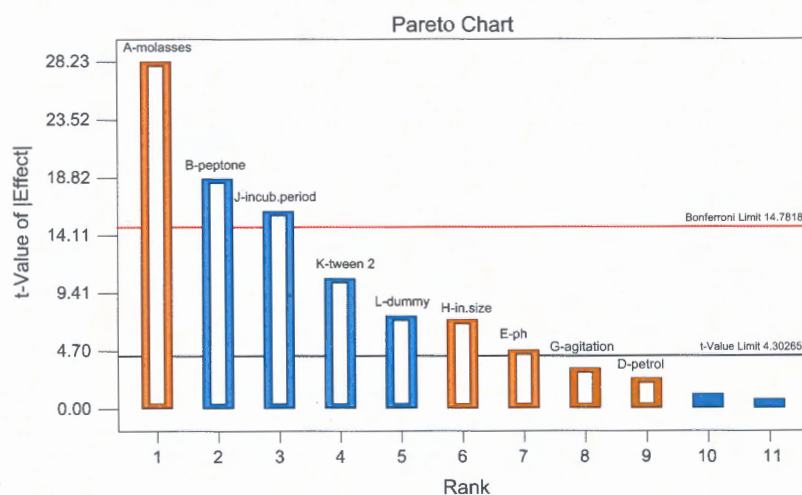
Fig. 5 Pareto chart showing the effect of media components on biosurfactant production.
