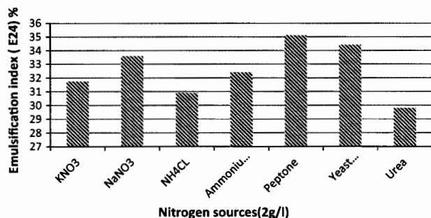
Fig. 3 Effect of nitrogen sources on biosurfactant production by Streptomyces isolate 5S.
