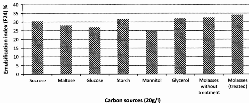
Fig. 2 Effect of carbon sources on biosurfactant production by Streptomyces isolate 5S.
