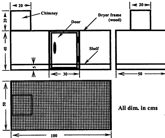
Figure (1): Schematic diagram of the solar dryer.
