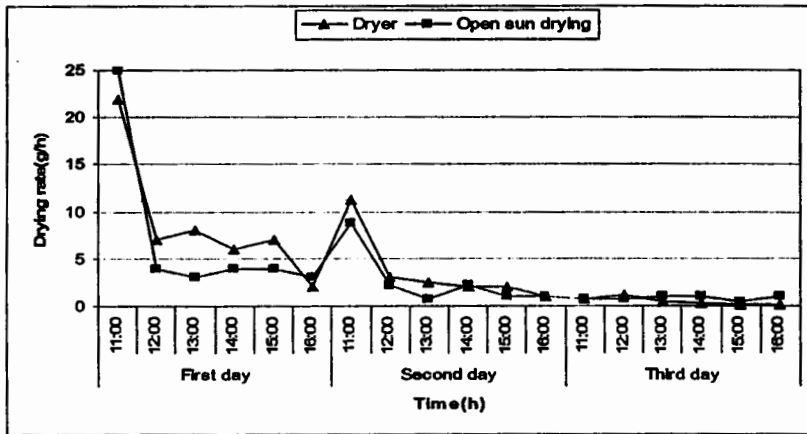
Figure (9) Variation of drying rate with drying time of okra in solar dryer and open sun.
