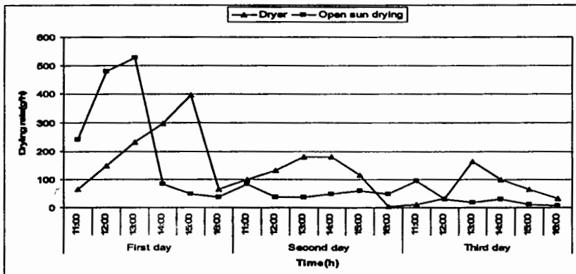
Figure(8) Variation of drying rate with drying time of grapes in solar dryer and open sun .
