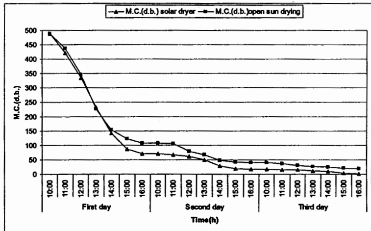
Figure (4) Variation of moisture content with drying time of mint in solar dryer and open sun.
