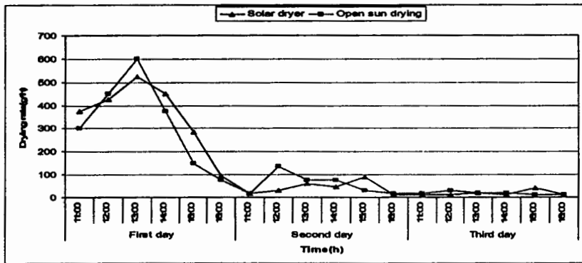
Figure(7) Variation of drying rate with drying time of mint in solar dryer and open sun .
