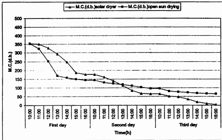
Figure (5) Variation of moisture content with drying time of grapes in solar dryer and open sun.
