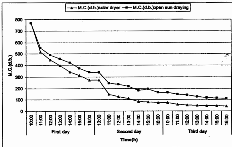
Figure (6) Variation of moisture content with drying time of okra in solar dryer and open sun.
