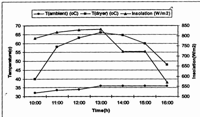
Figure (3) The variation of temperature in the dryer, ambient temperature and solar radiation intensity during (15 / 9 / 2013)
