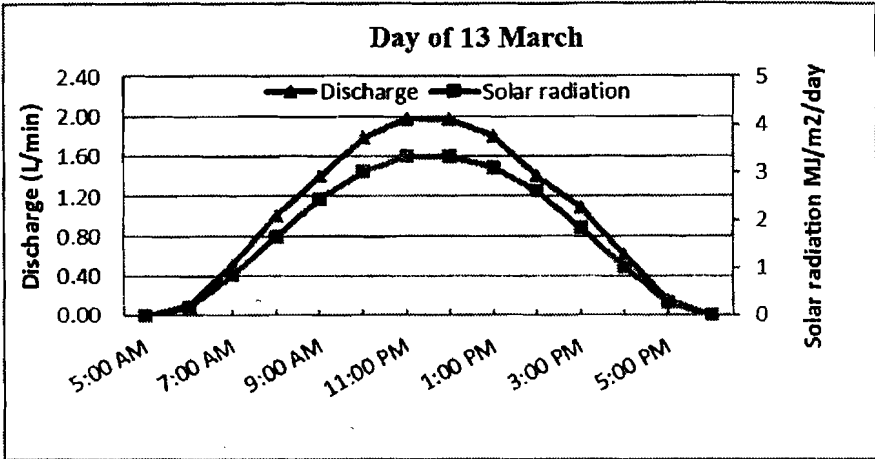
Fig.(11) The discharge with Hourly Average radiation for 13 March (hourly average radiation data were get from Meteorological Authority).
