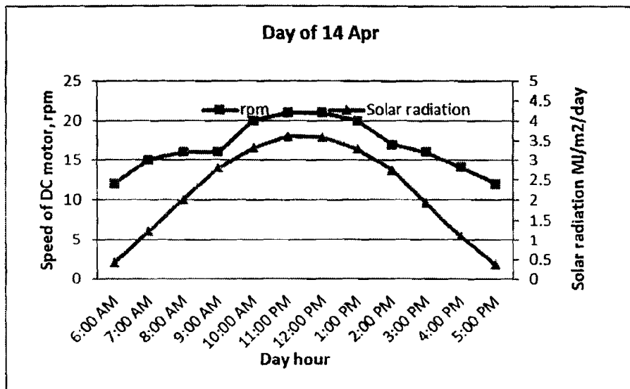
Fig.(15)Rpm values with hourly average radiation for 14 th April.
