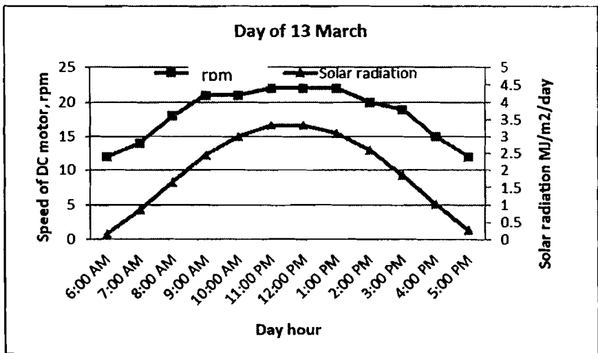
Fig.(14):Rpm value with hourly average radiation for 13 March
