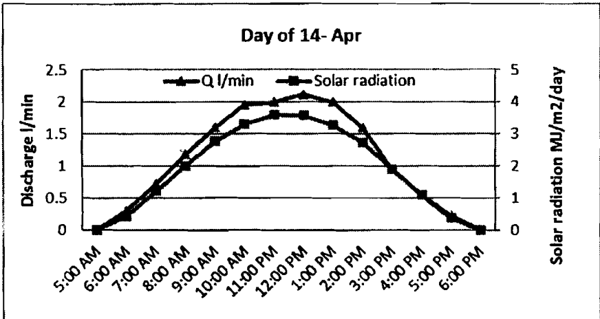
Fig.(12) The discharge with Hourly Average radiation for 14 April (hourly average radiation data were get from Meteorological Authority).
