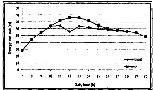
Fig (12): Variation of energy output (E) for PV with cooling and without cooling at daily hours.
