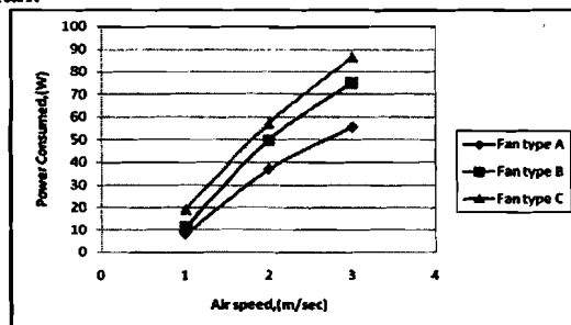
Figure (5): The relationship between power consumed, (W) for three types of fan blades and its air speeds (m/s).
