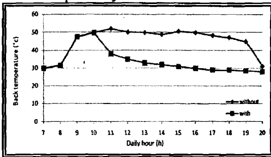
Fig (11): Variation of back temperature (°C) for PV with cooling and without cooling at daily hours.
