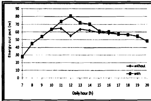
Fig (8): Variation of energy output (E) for PV with cooling and without cooling at daily hours.
