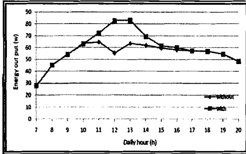
Fig (10): Variation of energy output (E) for PV with cooling and without cooling at daily hours.
