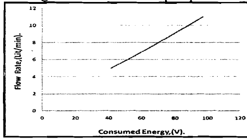
Figure (6): The relationship between consumed energy (E) and its pump speeds (Lit/min).
