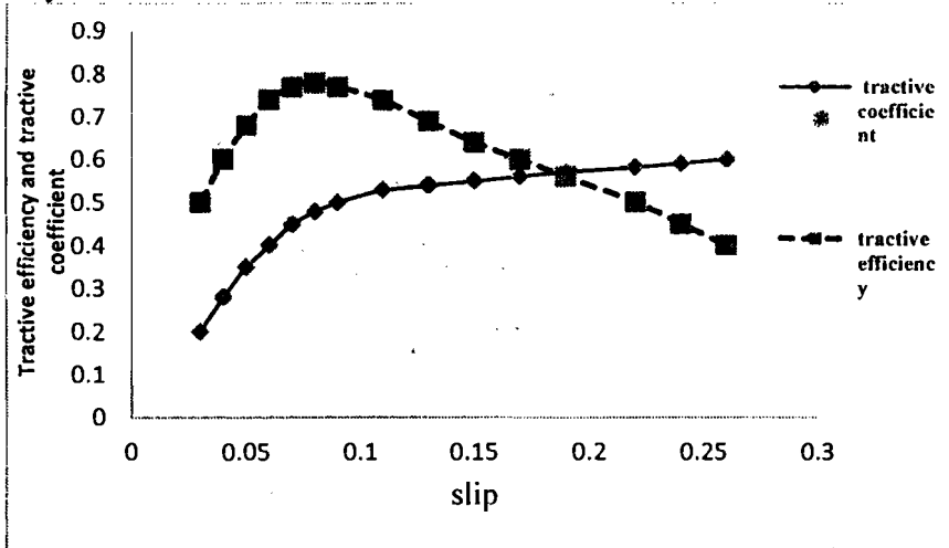
Fig.1: The relationship between tractive efficiency and tractive coefficient with slip.
