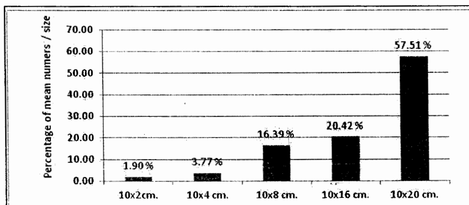
Figure (1): % capture of five tested trap size placed in both tomato and cabbage fields.
