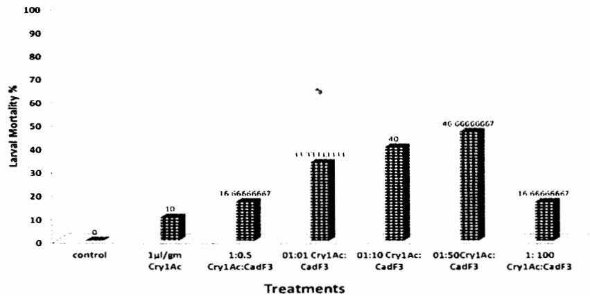
Fig. (5): Synergism effect of CadF3 fragment to BtCry1Ac toxin against the third larval instar of cotton leafworm.
