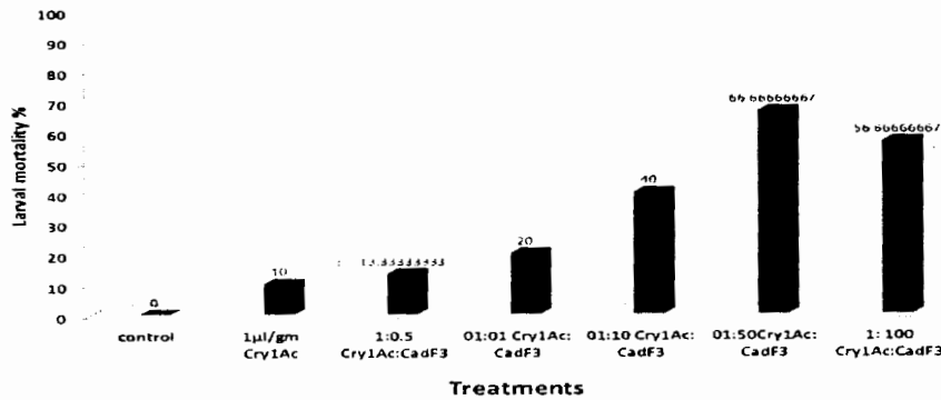
Fig. (4): Synergistic effect of CadF3 fragment to BtCry1Ac toxin against the second larval instar of cotton leafworm.
