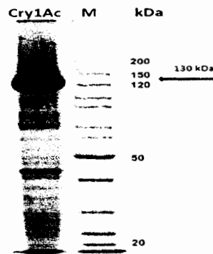
Fig.1: SDS-PAGE electrophoresis of Cry1Ac partially purified toxin, M: Represents PageRoler marker, Lanes 1, 2 and 3: Represent 10, 10 and 20ul of Cry1Ac loaded
