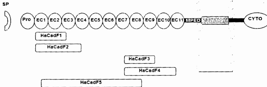
Fig. (2): Diagram of H. armigera cadherin receptor and its various domains. SP: Represents signal peptide; Pro: Represents propeptide region; EC: Represents ectodomain regions; MPED: Represents membrane-proximal extracellular domain; CYTO: Represents cytoplasmic domain; HaCadF: Represents recombinant proteins of cadherin fragments (CadF1, CadF2, CadF3, CadF4, and CadF5)
