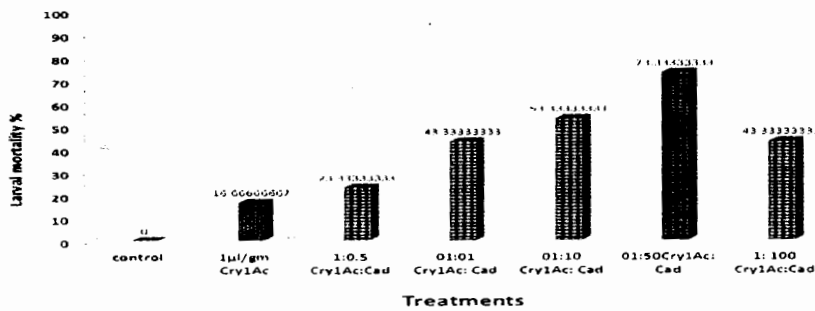
Fig. (3): Synergistic effect of CadF3 fragment to BtCry1Ac toxin against the first larval instar of cotton leafworm.
