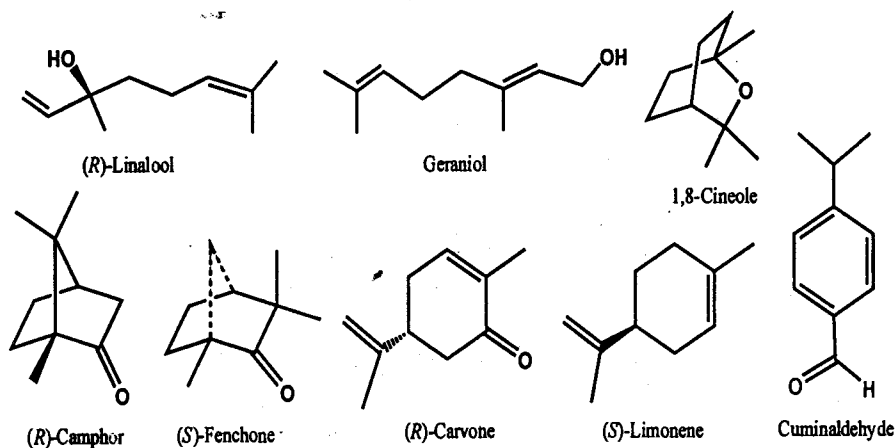
Figure 1. The chemical structures of the tested monoterpenes.
