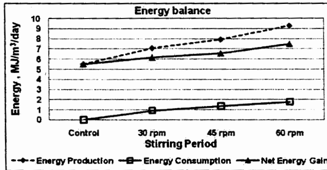
Fig.(8): The average energy balance at different stirring speeds
