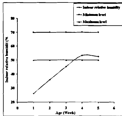
Fig (3) Weekly indoor air relative humidity
