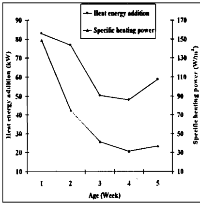
Fig (5) relation between heat energy addition and specific heating power during birds age
