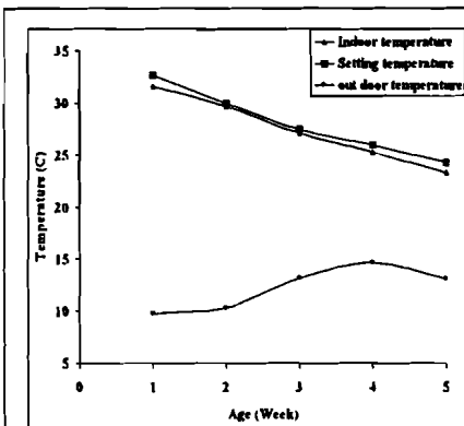
Fig (1) Weekly average indoor air temperature
