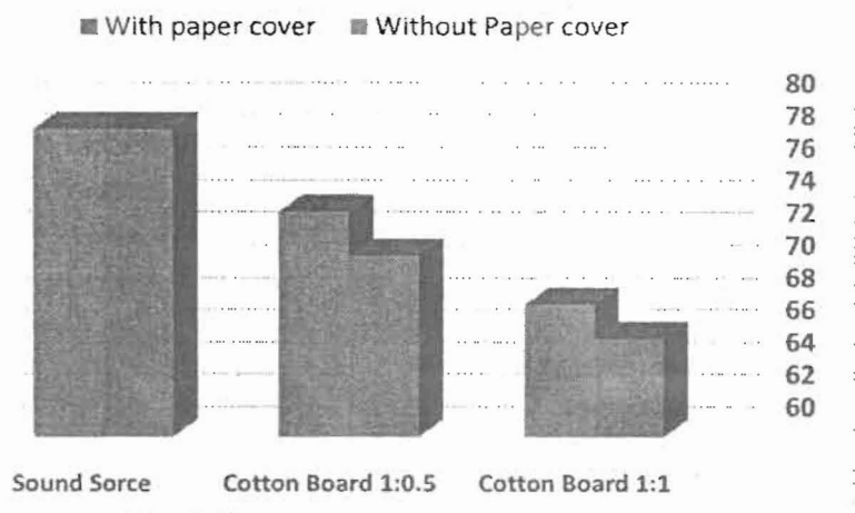
Fig (4) The effect of mixing ratio on the insulation performance for Cotton Stalks
