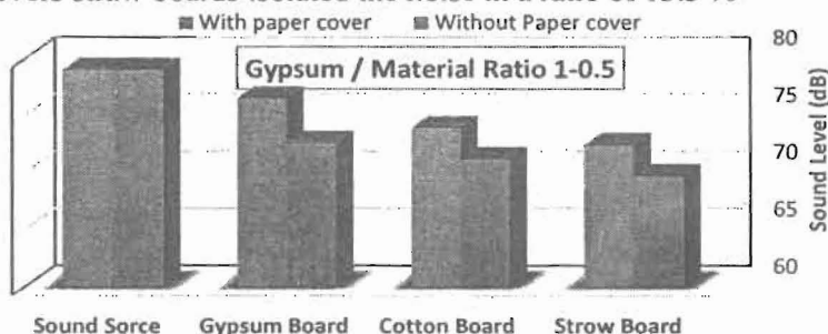
Fig (1) The effect of residual kind on the insulation performancefor Gypsum / material ratio of 1: 0.5
