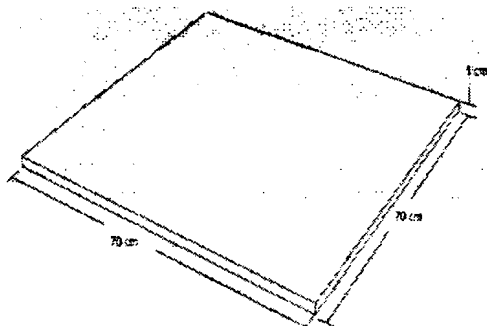
Fig. (1) The Gypsum board dimension
