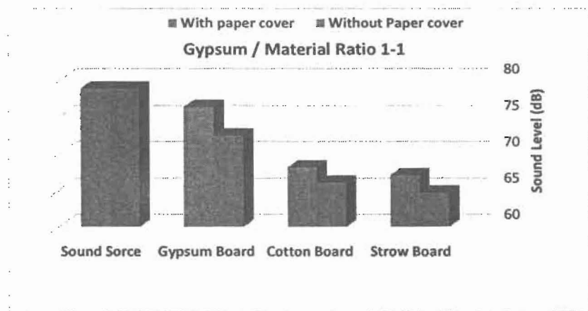
Fig (2) The effect of residual kind on the insulation performance for Gypsum / material ratio of 1: 1
