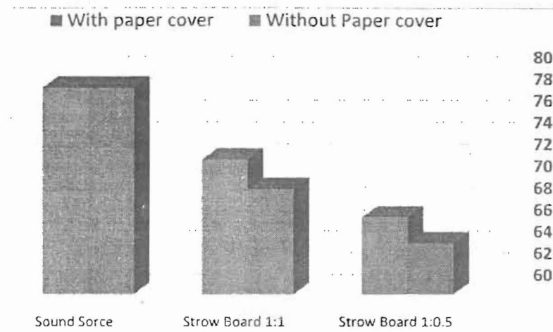
Fig (3) The effect of mixing ratio on the insulation performance for Straw
