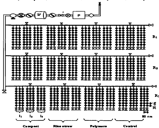
Fig. 1. Schematic hydraulic diagram of the micro irrigation system and treatments
