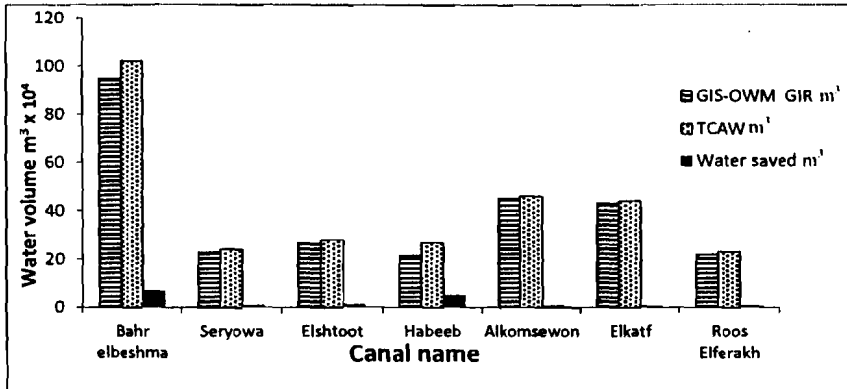
Figure (4): Irrigation water allocation using GIS-OWM among the canals on rotation NO. 21
