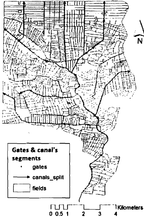
Figure (1): Segments and gates distribution
