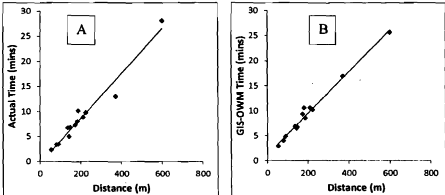
Figure (2): The relationships between the distance among gates (m) and each of actual consumed time (mins) (A) and calculated from GIS-OWM model (mins) (B).
