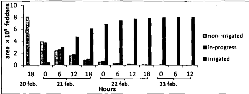
Figure (7): Areas per (feddans) for field irrigation status per 6 hours
