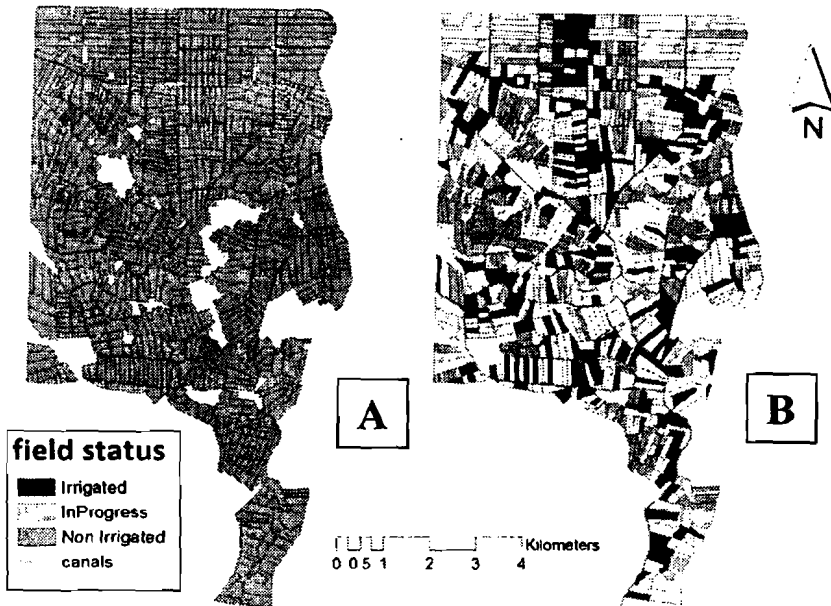
Figure (5): GIS-OWM for field irrigation status dynamic map on (A) 20 Feb. at 6 pm, (B) 21 Feb at 6 am
