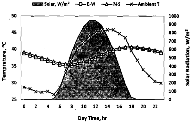
Fig. (11): Hourly average temperatures (north-south and east-west directions, and ambient air) and solar radiation intensity during the experimental period.
