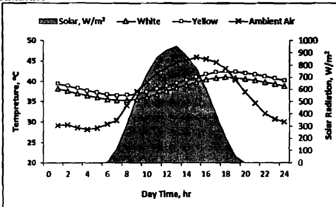
Fig. (10): Hourly average temperatures (white and yellow colors, and ambient air) and solar radiation intensity during the experimental period.
