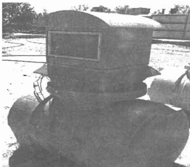
Fig. (16): Two identical water storage tanks; one equipped with fan and the other without fan.
