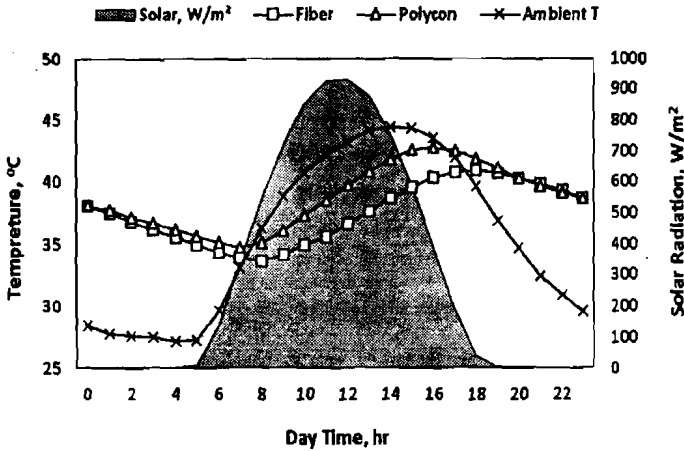
Fig. (14): Hourly average temperatures (polyethylene and fibreglass storage tanks, and ambient air) and solar radiation intensity during the experimental period.
