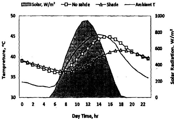
Fig. (15): Hourly average temperatures (with shading screen and without shading storage tanks, and ambient air) and solar radiation intensity during the experimental period.
