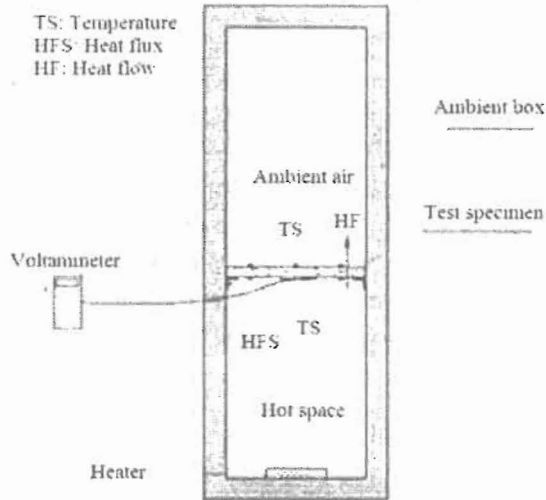
Fig. (6): Schematic diagram of the test set-up
