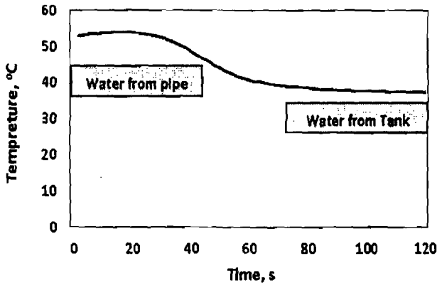
Fig. (18): Hourly average water temperatures just leaving the storage tank and draining from the pipes network.
