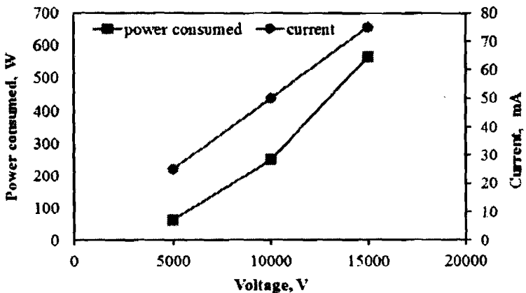
Fig. 3: shows the power consumption and electrical current for high voltage levels.
