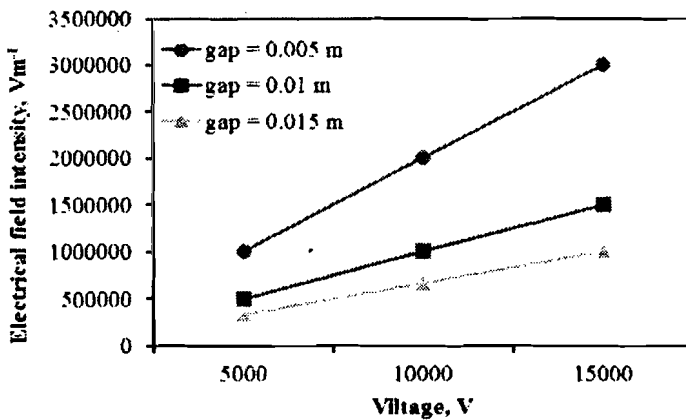
Fig. 4: shows the electrical field intensity at high voltage 5000, 10000 and 15000 V for electrode gap 0.5, 1 and 1.5 cm.
