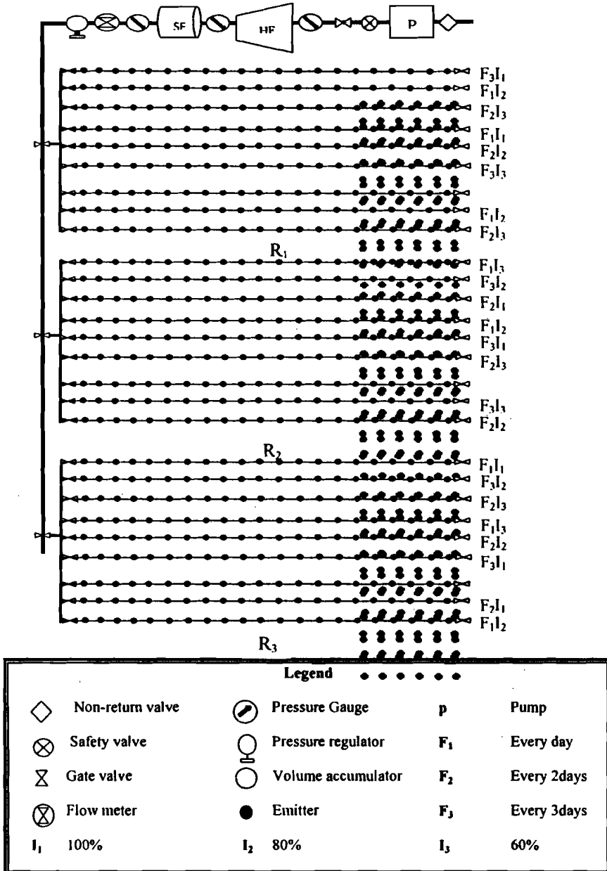
Fig. 1. Layout of an experimental design that includes three irrigation frequencies and three irrigation rates.
