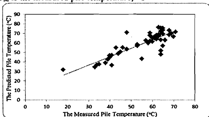
Figure (6): The comparison between the predicted and the measured temperatures of compost pile during the whole period of compost.
