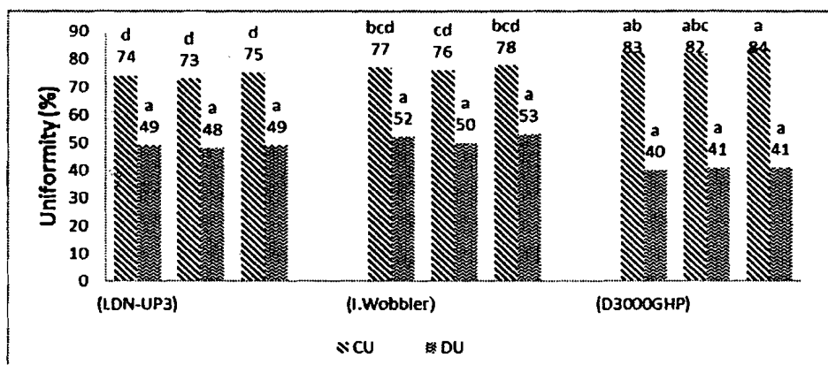
Fig. 6. Average CU and DU values of the three sprinkler types.
