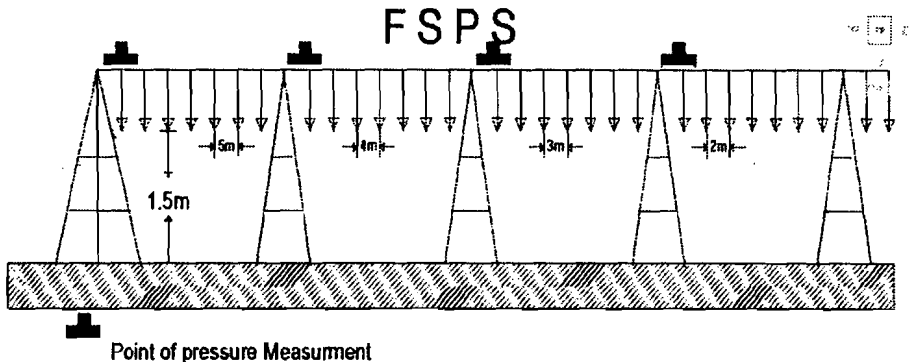
Fig.1. Diagram of the positioning of sprinklers on the center pivot system.
