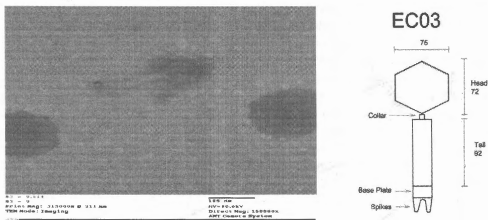
Fig. 2. Schematic diagram and electron micrograph of negatively stained phage Ec03. The bar represents 100nm
