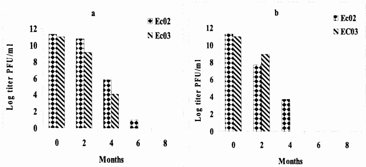
Fig. 7. The effect of storage period on the maintenance of phage suspension at a-refrigerator (4°C) and b-freezer conditions (-20°C)
