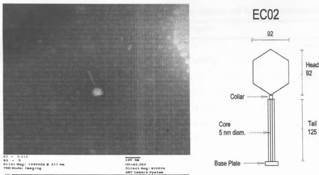
Fig. 1. Schematic diagram and electron micrograph of negatively stained phage Ec02. The bar represents 100 nm.
