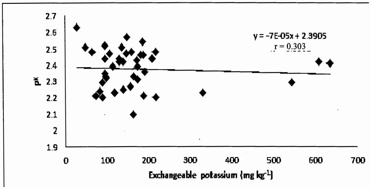
Fig. 2. Relationship between exchangeable potassium and potassium potential in the investigated soils
