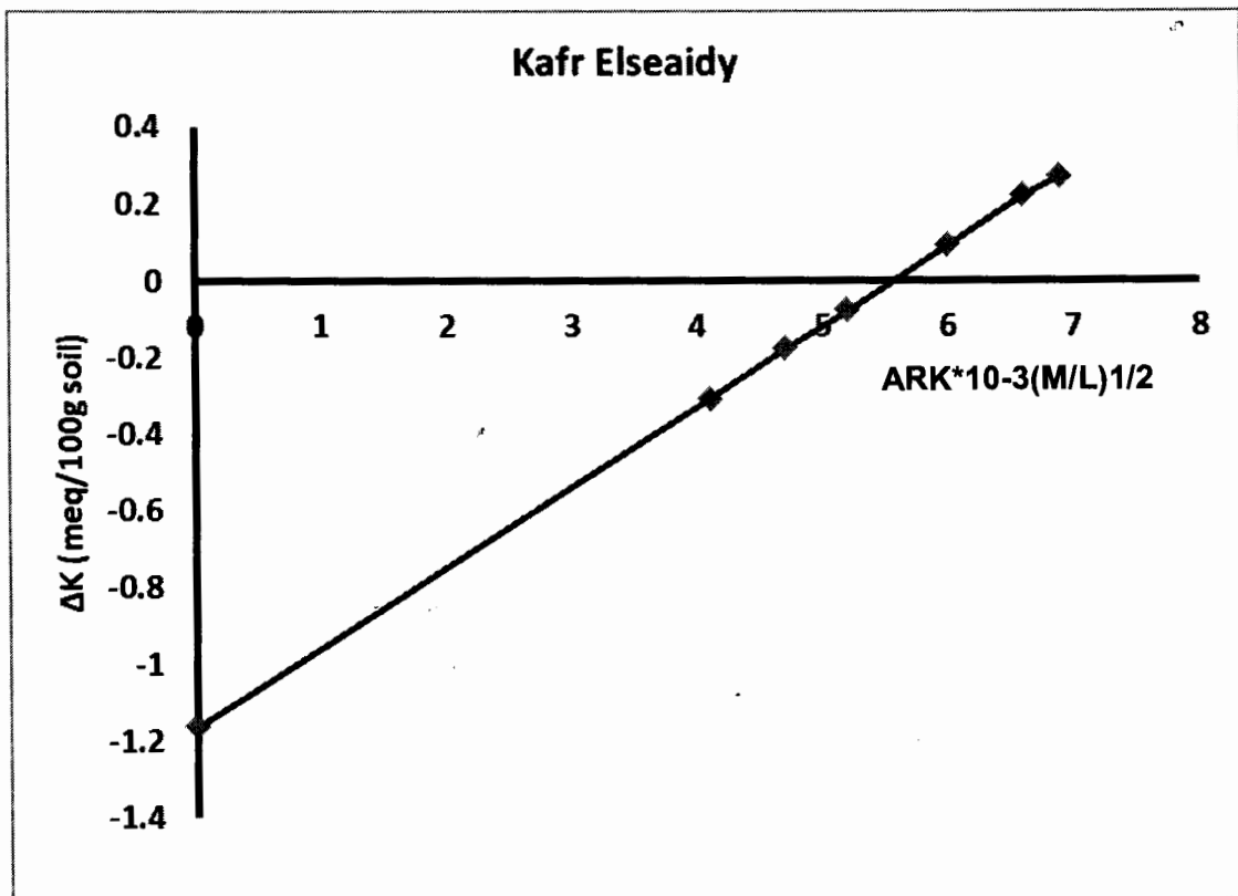
Fig. 3 The Q/I curve of Ezbt Elgendy and Kafr Elseaidy
