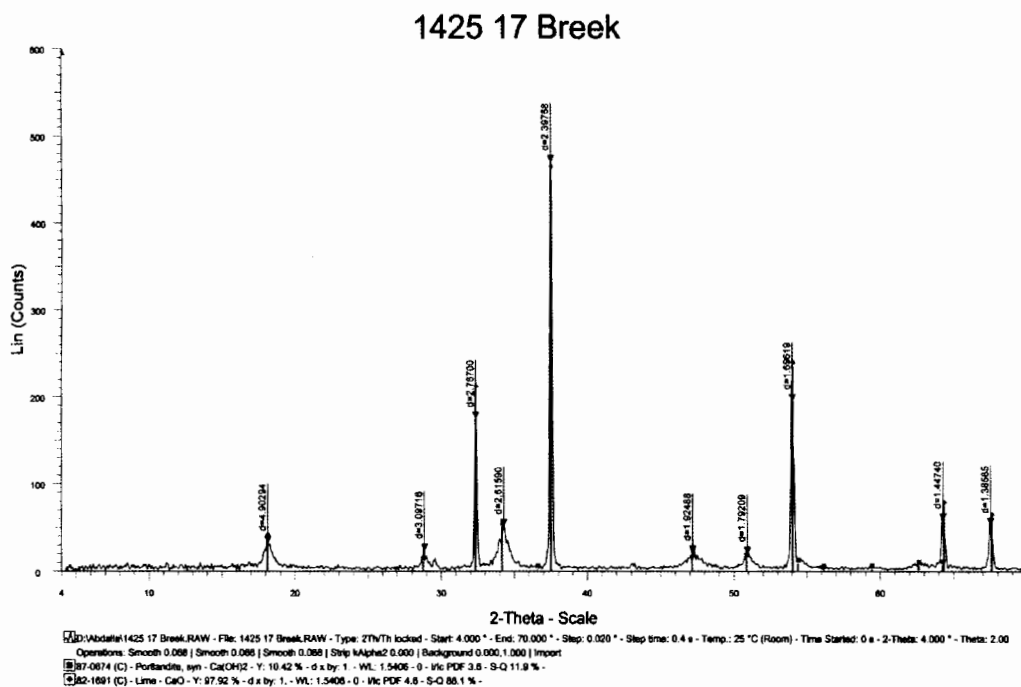
Fig. 1. XRD peak patterns and the phase transformation of chicken eggshells calcinated from 300° C to 900° C for 1h.
