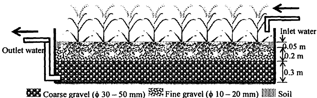
Fig. 1. Schematic diagram of the constructed wetland
