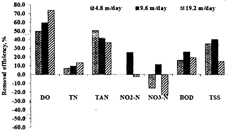
Fig. 2: Wetland nutrient removal efficiency at different hydraulic loading rates.
