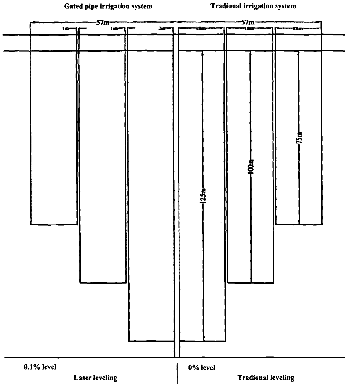
Fig. 1. Experiment layout
