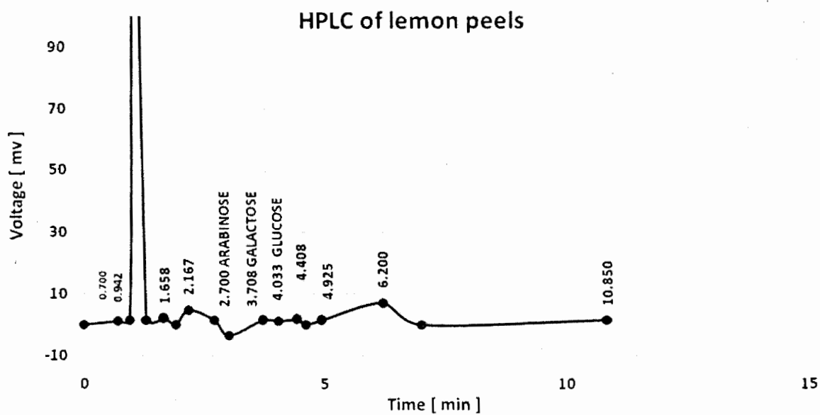
Fig. 3. HPLC of lemon peels
