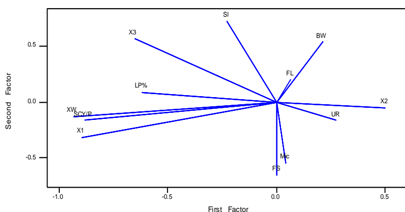
Fig. I. Plot of the first tow PCs as showing relation among variance characters in F_3 generation
